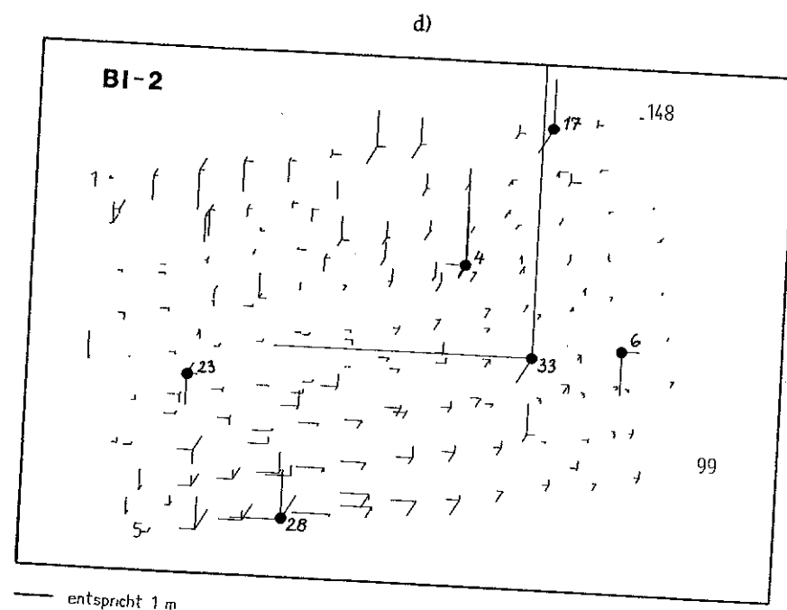
Figure 19 — (continued) True Errors of Bundle Blocks B I/2
