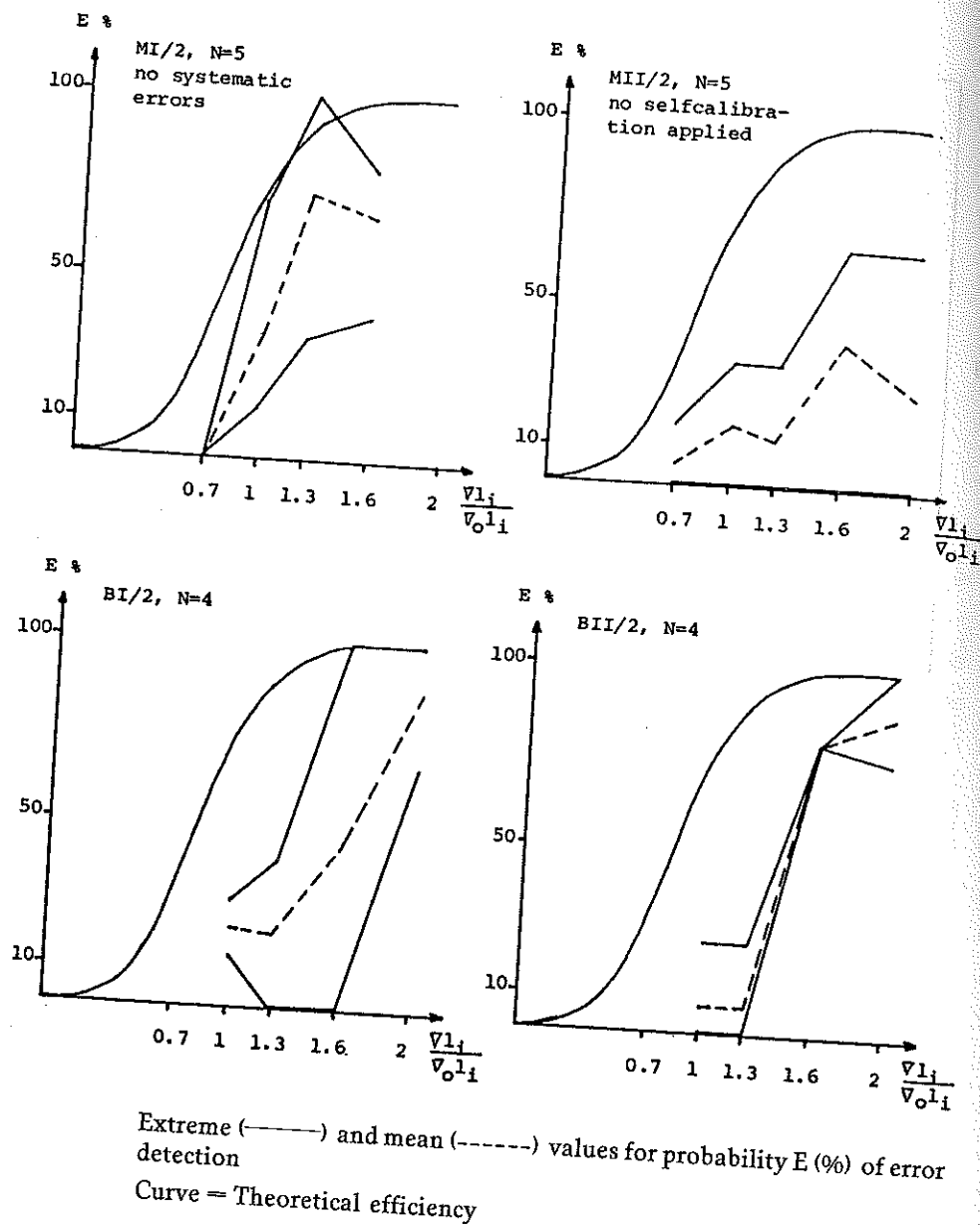
Figure 18 — Empirical and Theoretical Efficiency of Practical Procedures (cf. Table 26)
