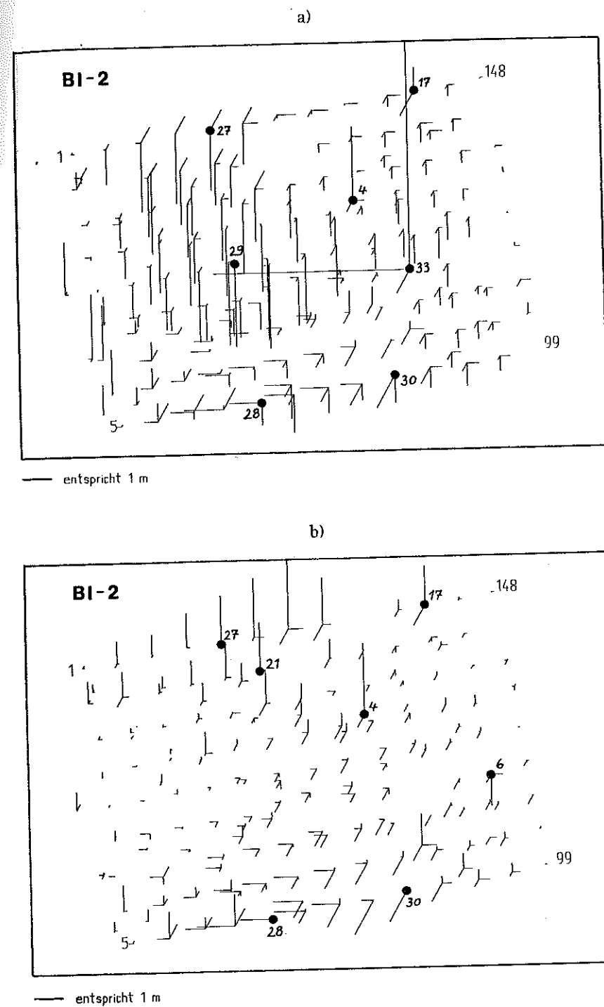
Figure 19 — True Errors of Bundle Blocks B I/2
