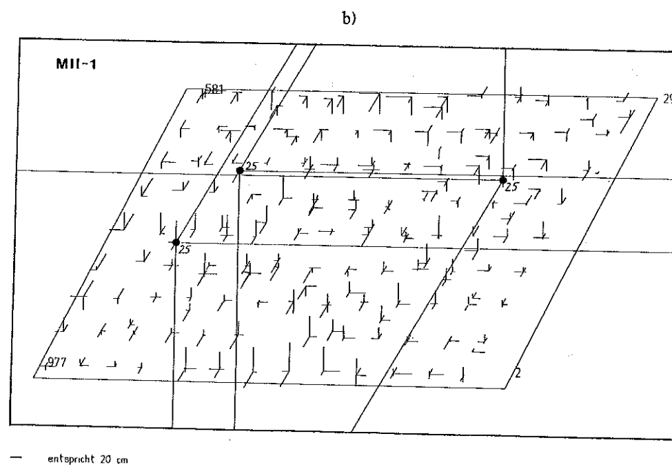
Figure 15 — True Errors of Model Blocks M II/1
