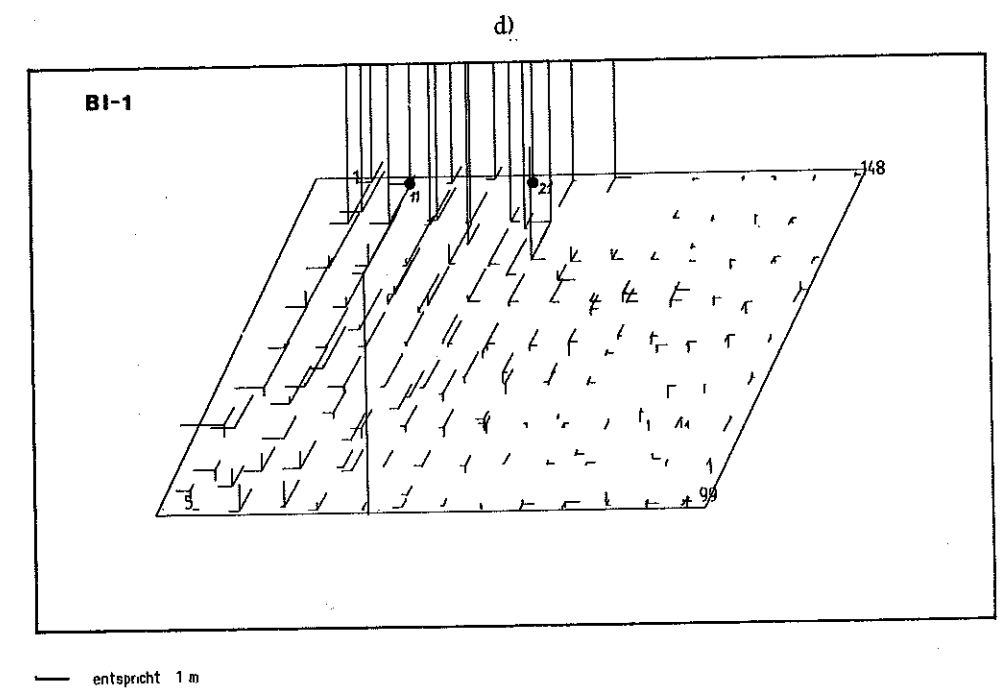
Figure 16 — (continued) True Errors of Bundle Blocks B I/1
