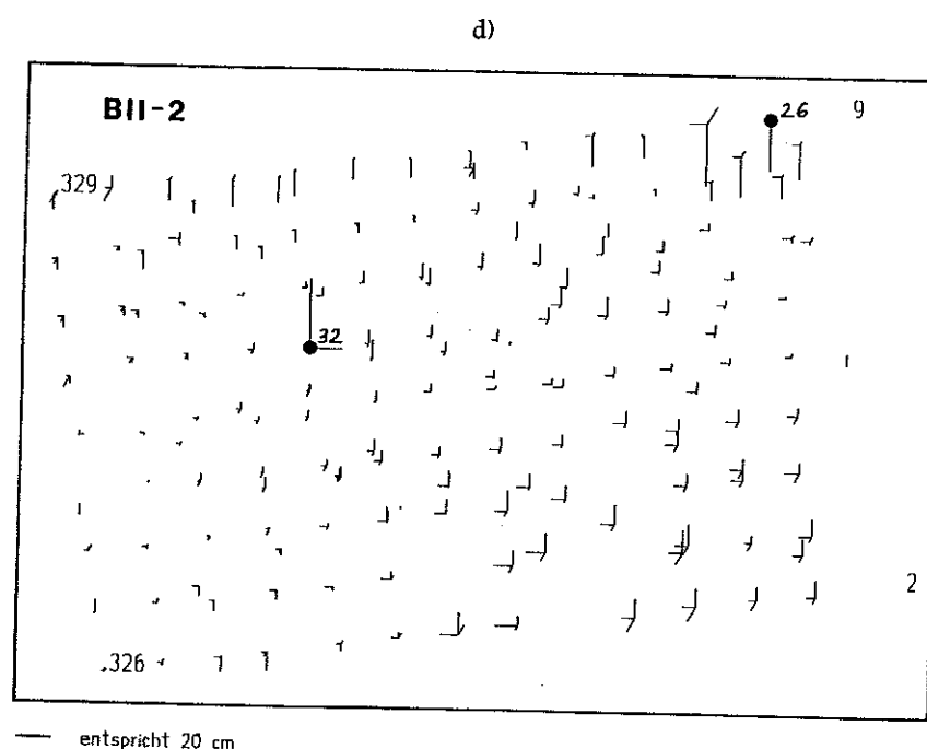
Figure 20 — (continued) True Errors of Bundle Blocks B II/2
