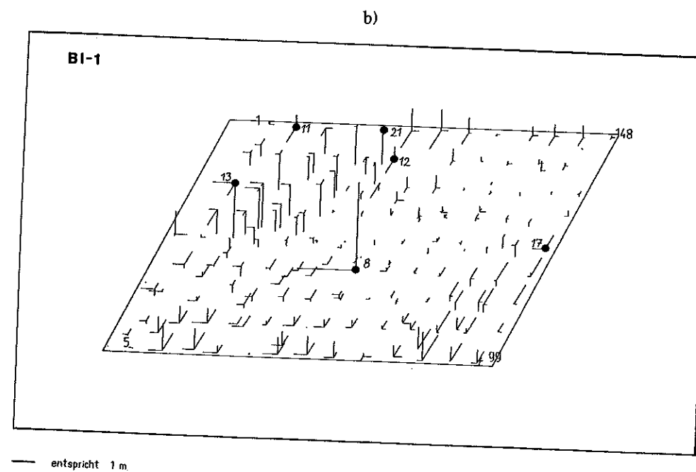
Figure 16 — True Errors of Bundle Blocks B I/1
