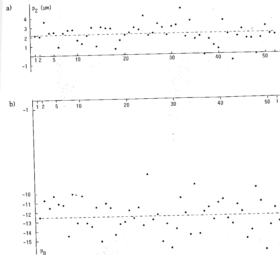
Figure 10 — Additional Parameters for Bundle Block B I/2
