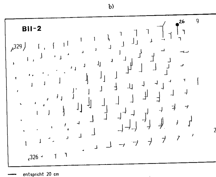
Figure 20 — True Errors of Bundle Blocks B II/2
