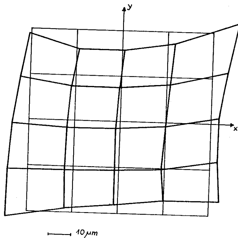
Figure 9 — Image Deformation of B II/1, Strips 1 and 2
